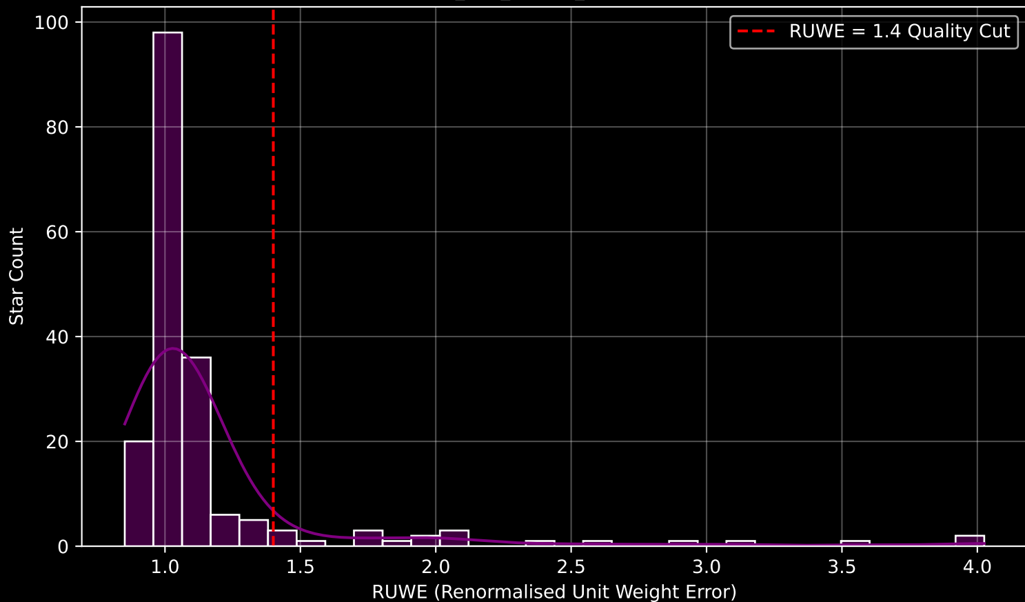
GAPOGEE DR17 Field [K2_C13_174-14_btx] RUWE Distribution (n= 185)
