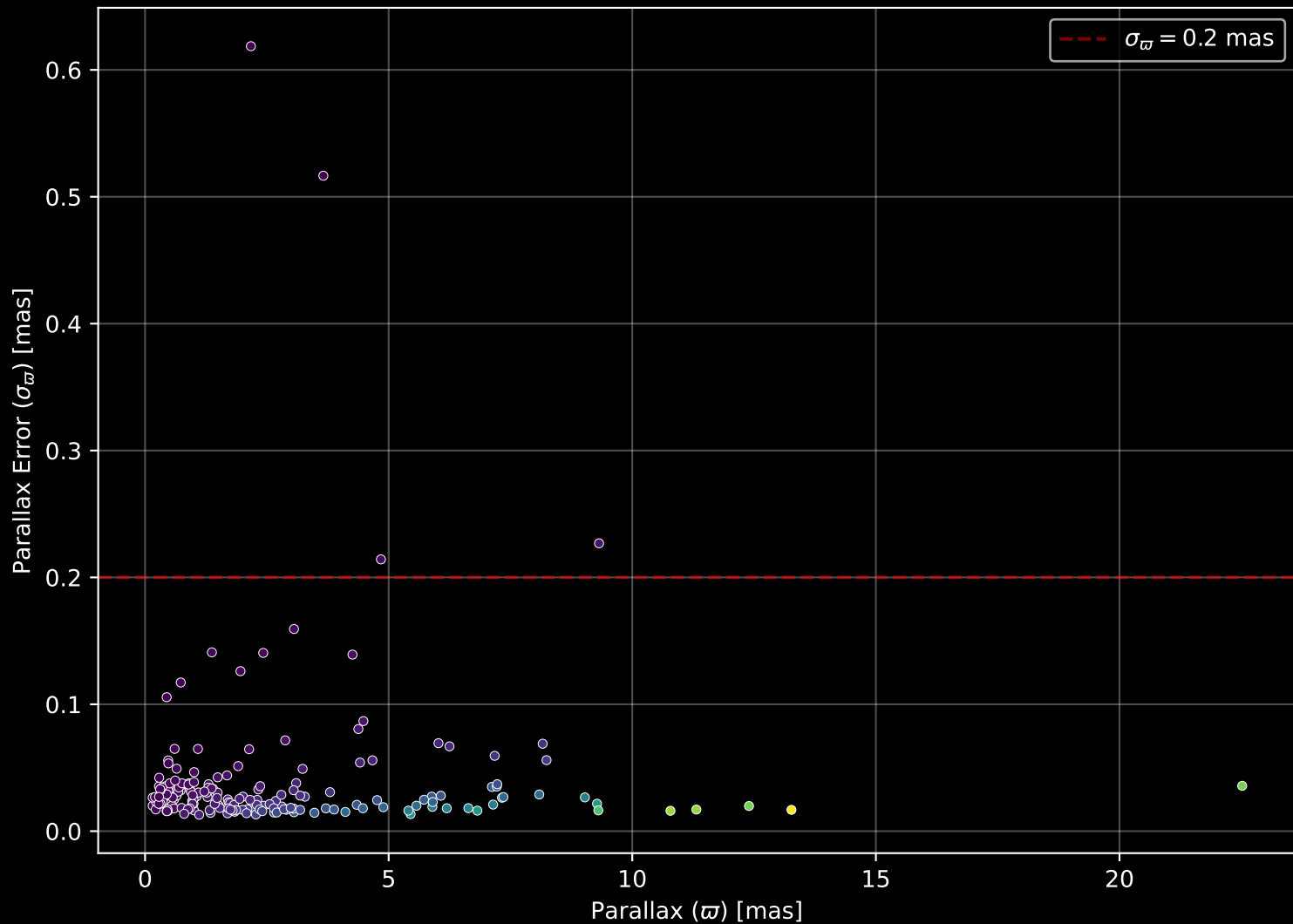
APOGEE DR17 Field: [K2_C13_174-14_btx] Parallax Quality (n= 191)
