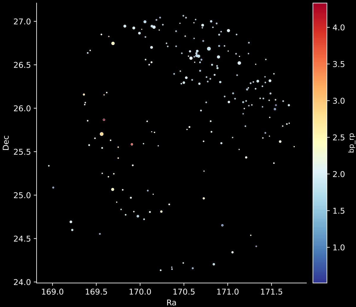
APOGEE DR17 Field: [K2_C13_174-14_btx] Stars: 191
