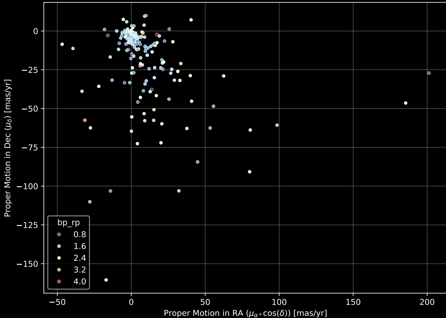
APOGEE DR17 Field: [K2_C13_174-14_btx] Proper Motion Diagram (n= 191)
