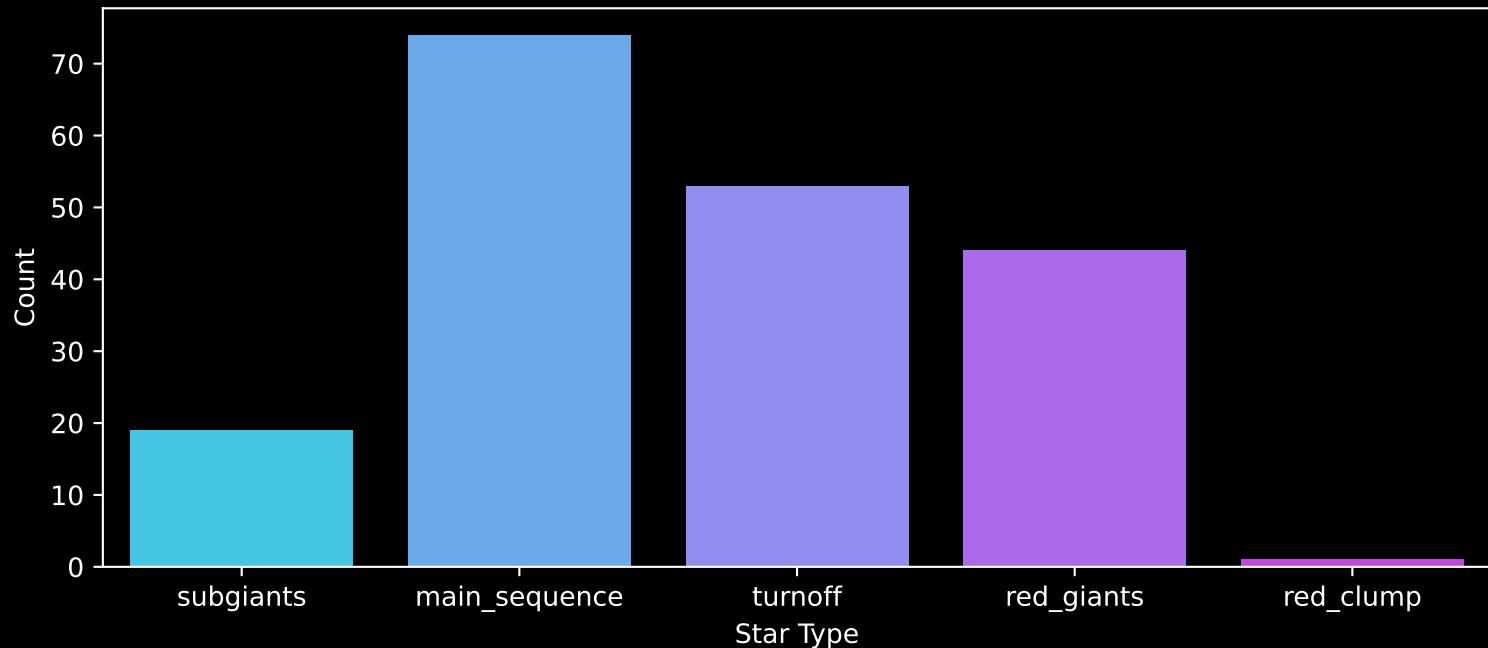
APOGEE DR17 Field: [K2_C13_174-14_btx] Count plot of Star Type
