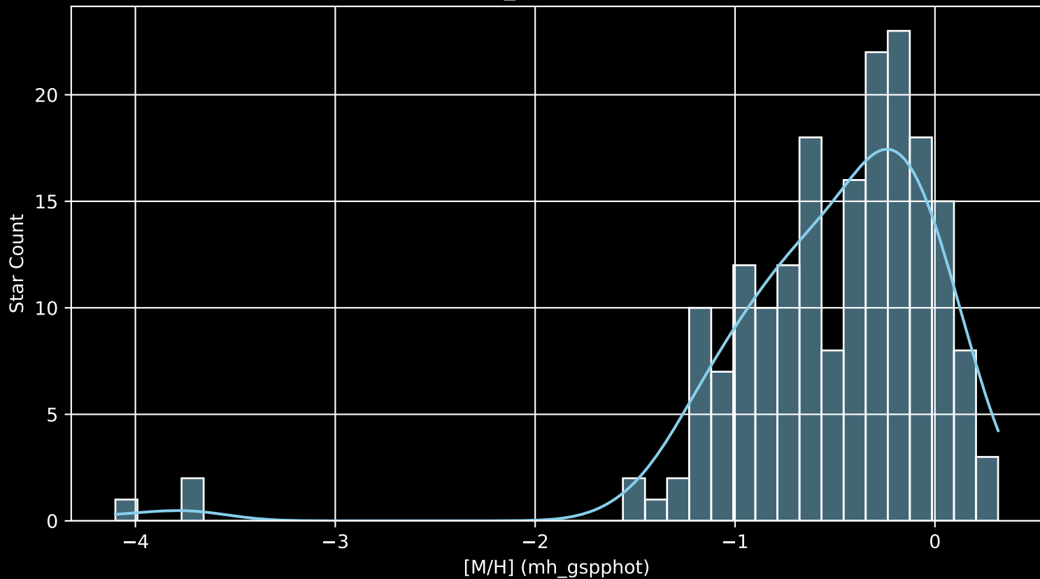
APOGEE DR17 Field: [K2_C13_174-14_btx [M/H] (mh_gspphot) (n= 190)
