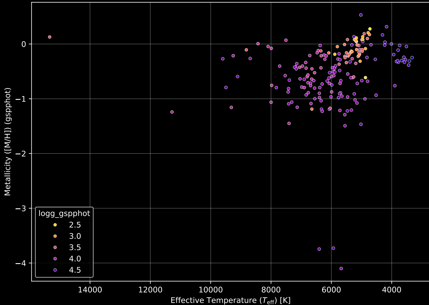
APOGEE DR17 Field: [K2_C13_174-14_btx] Stellar Population Parameters (n= 191)
